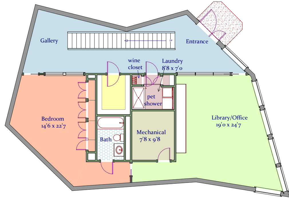
Level 1 - 1692 square feet +/- 1618 finished square feet +/- 74 unfinished square feet +/-
